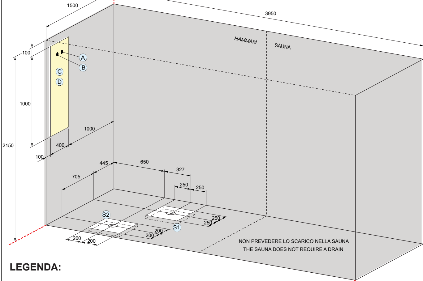
S1: SCARICO VASCA / TAB DRAIN
